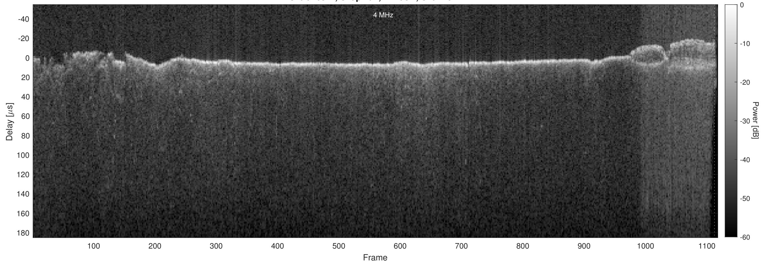
Orbit 16342, Chapman, Window, Channel 2
