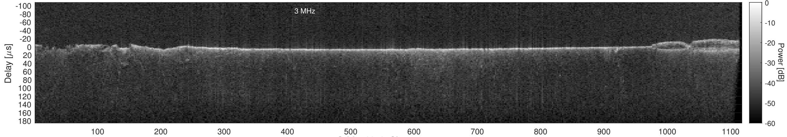
Orbit 16342, Cluttergram
