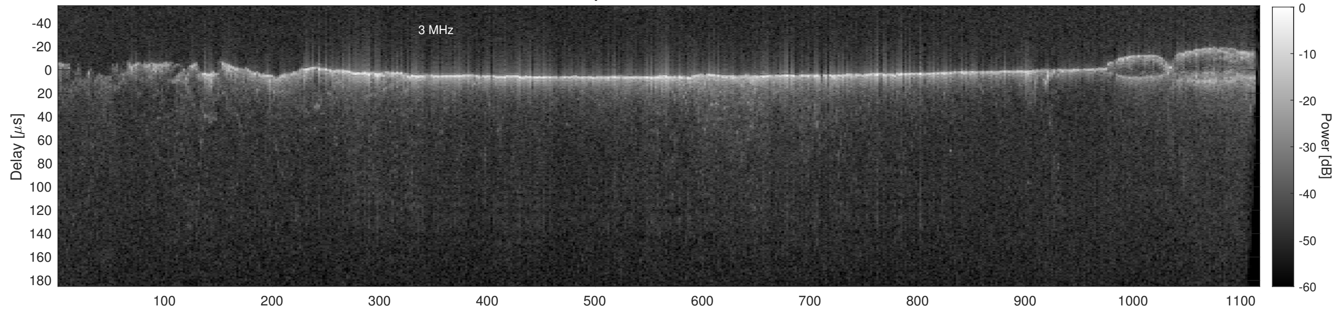
Orbit 16342, Cluttergram
