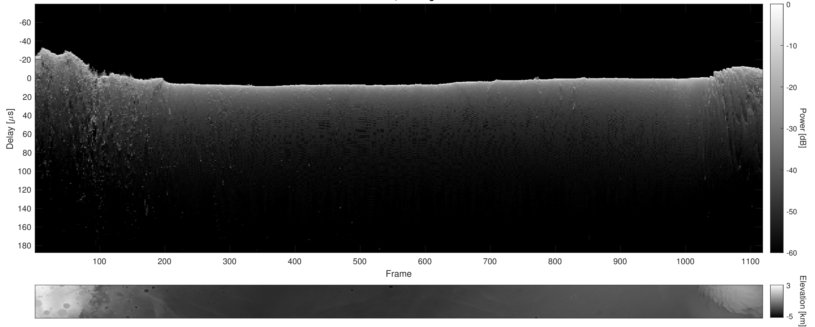
Orbit 16344, Cluttergram
