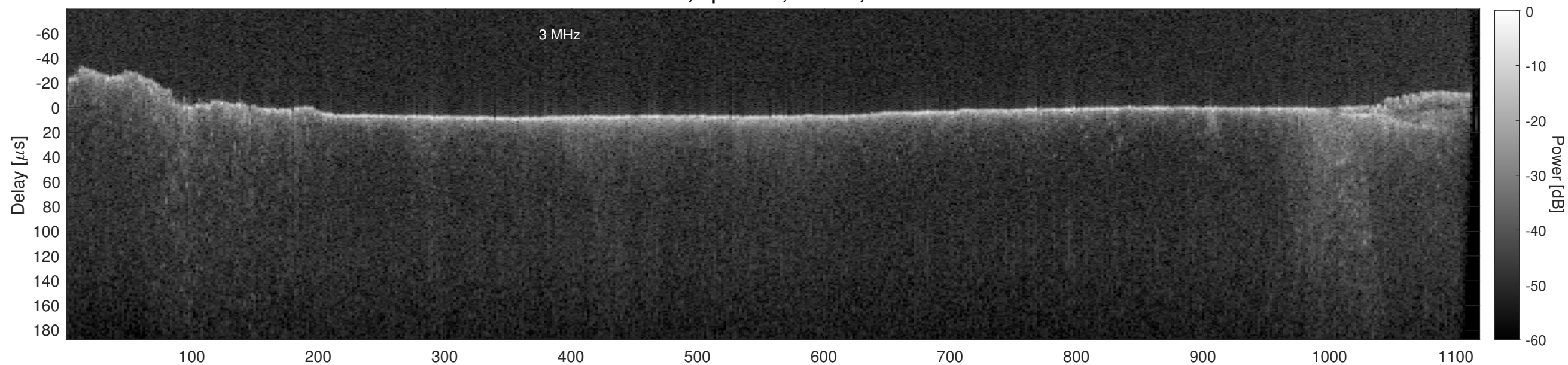
Orbit 16344, Cluttergram
