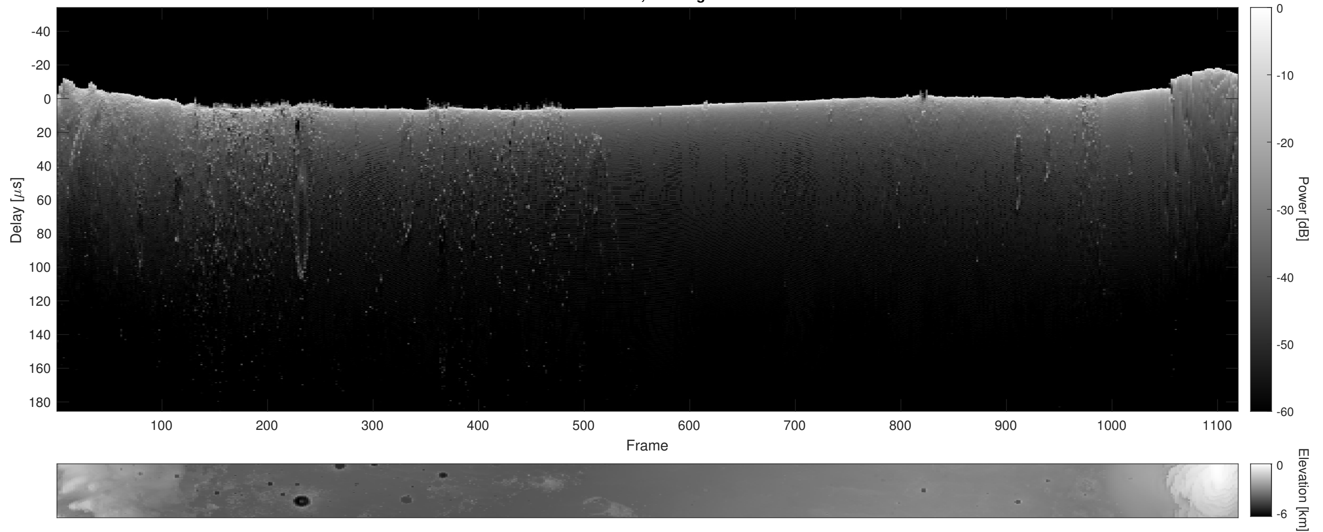
Orbit 16354, Cluttergram
