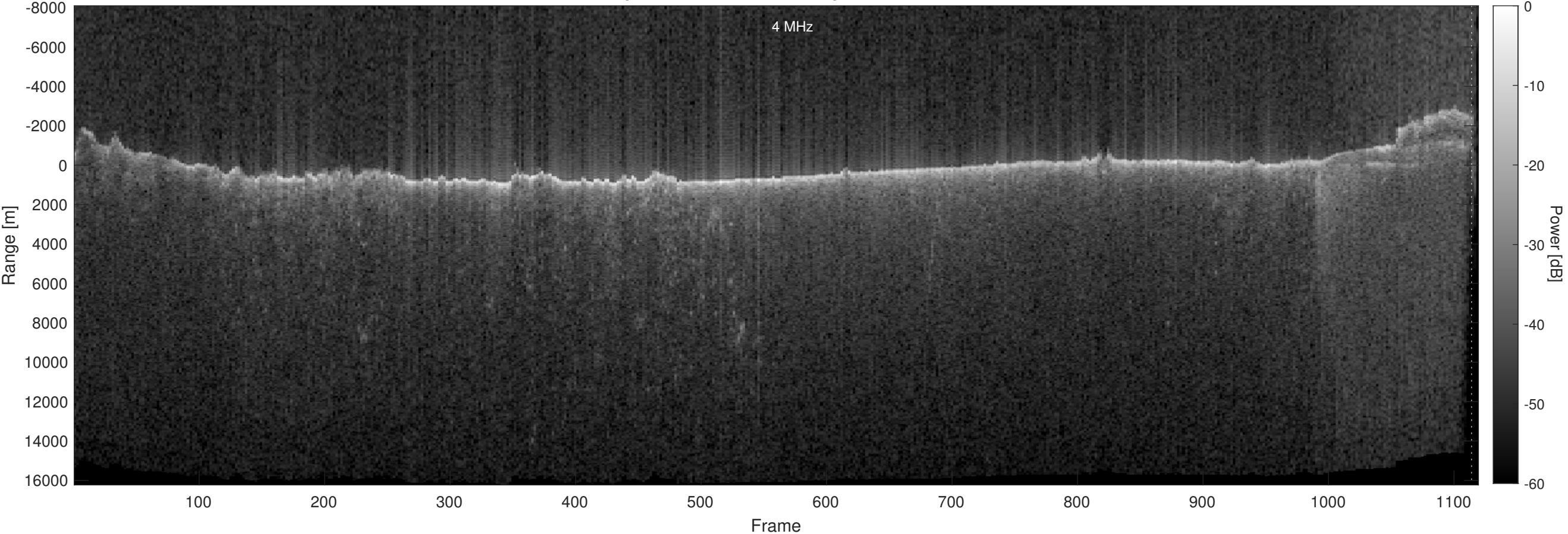
Orbit 16354, Optimized, No Window, Depth-Corrected, Channel 2
