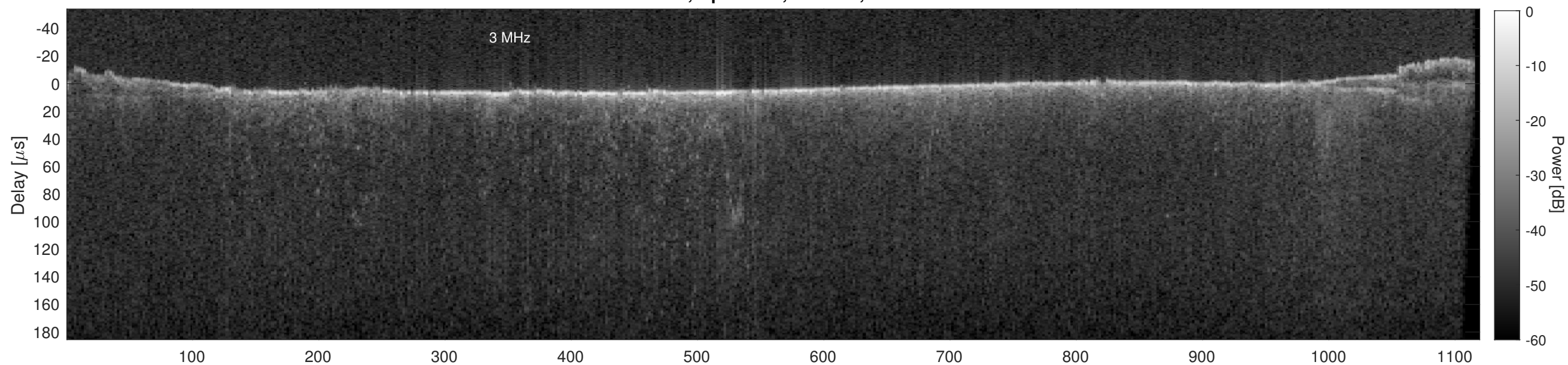
Orbit 16354, Cluttergram
