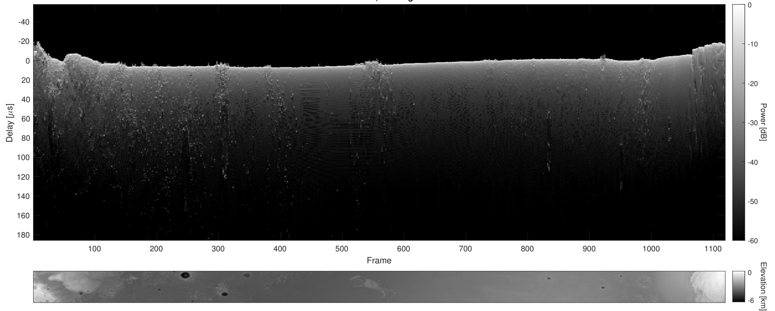
Orbit 16361, Cluttergram
