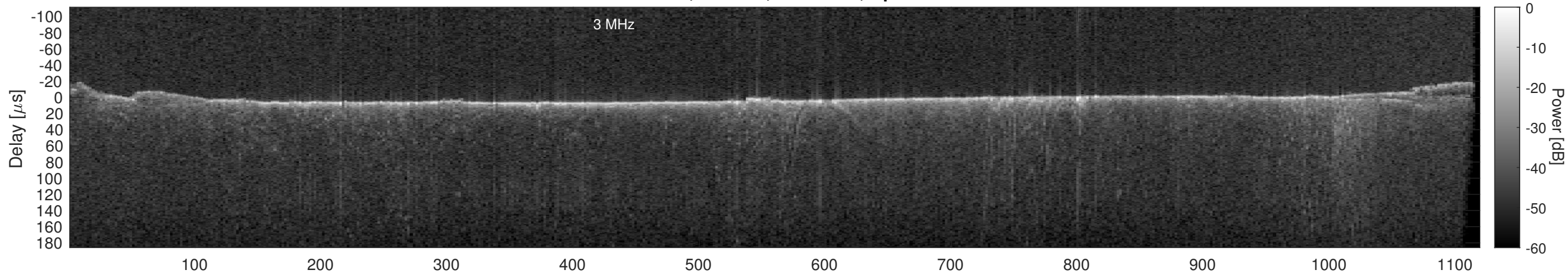
Orbit 16361, Cluttergram
