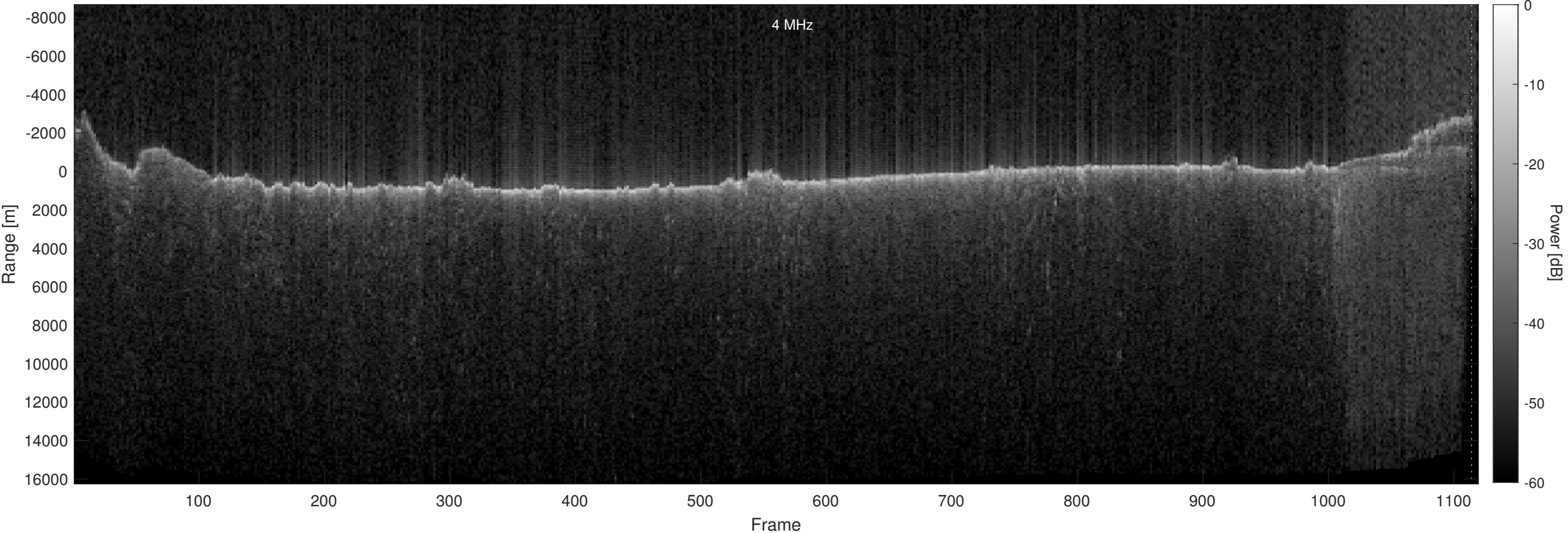
Orbit 16361, Optimized, No Window, Depth-Corrected, Channel 2
