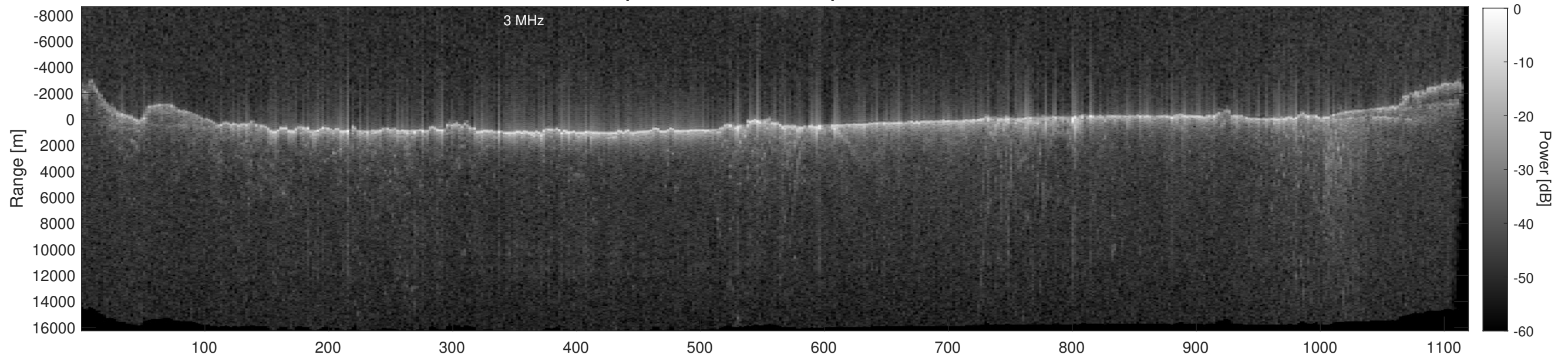
Orbit 16361, Depth-Corrected Cluttergram
