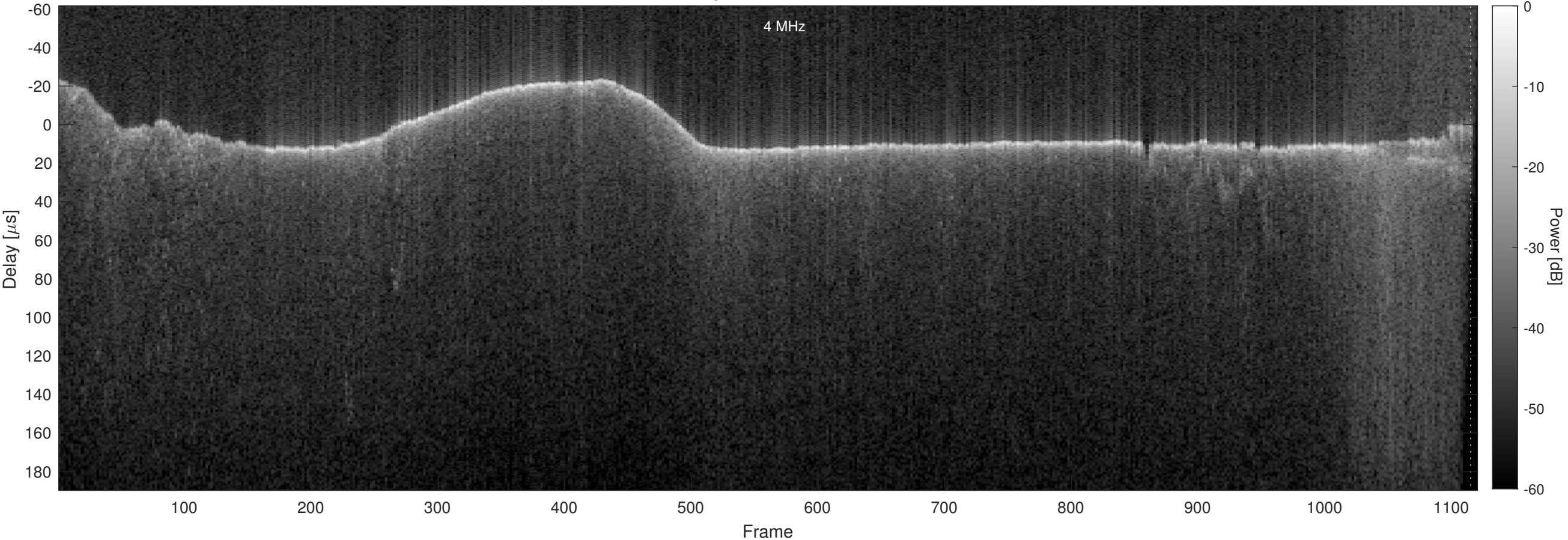
Orbit 16372, Chapman, No Window, Channel 2
