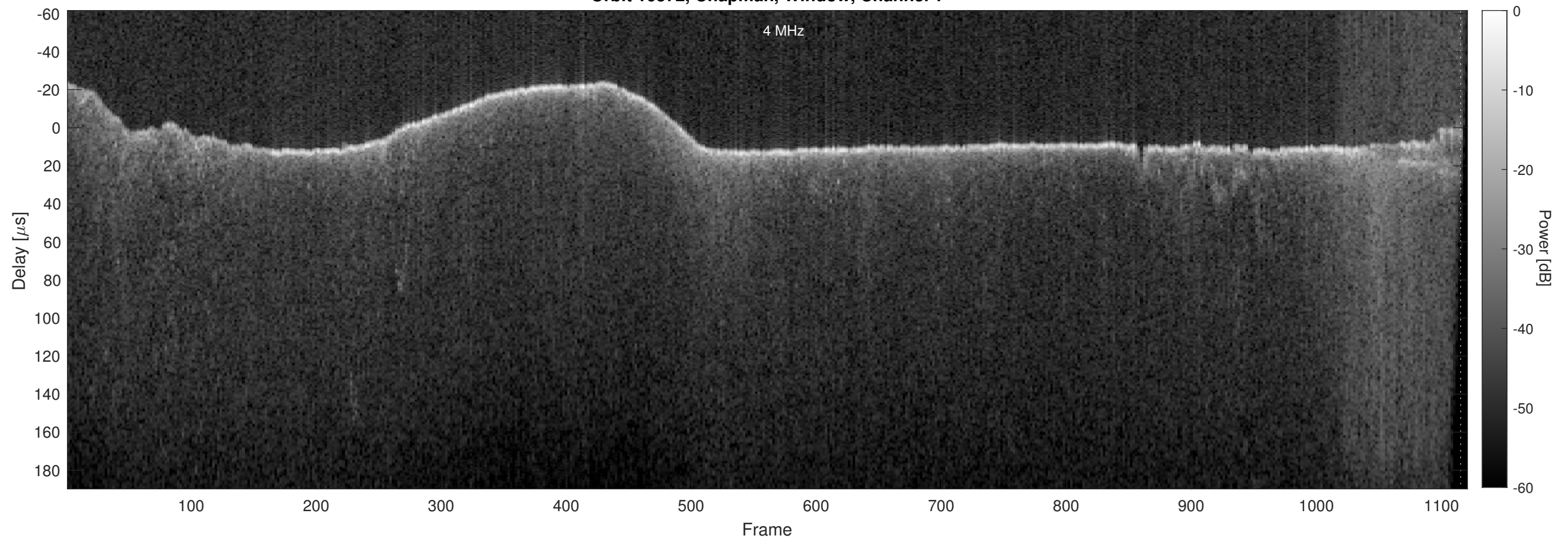
Orbit 16372, Chapman, Window, Channel 2
