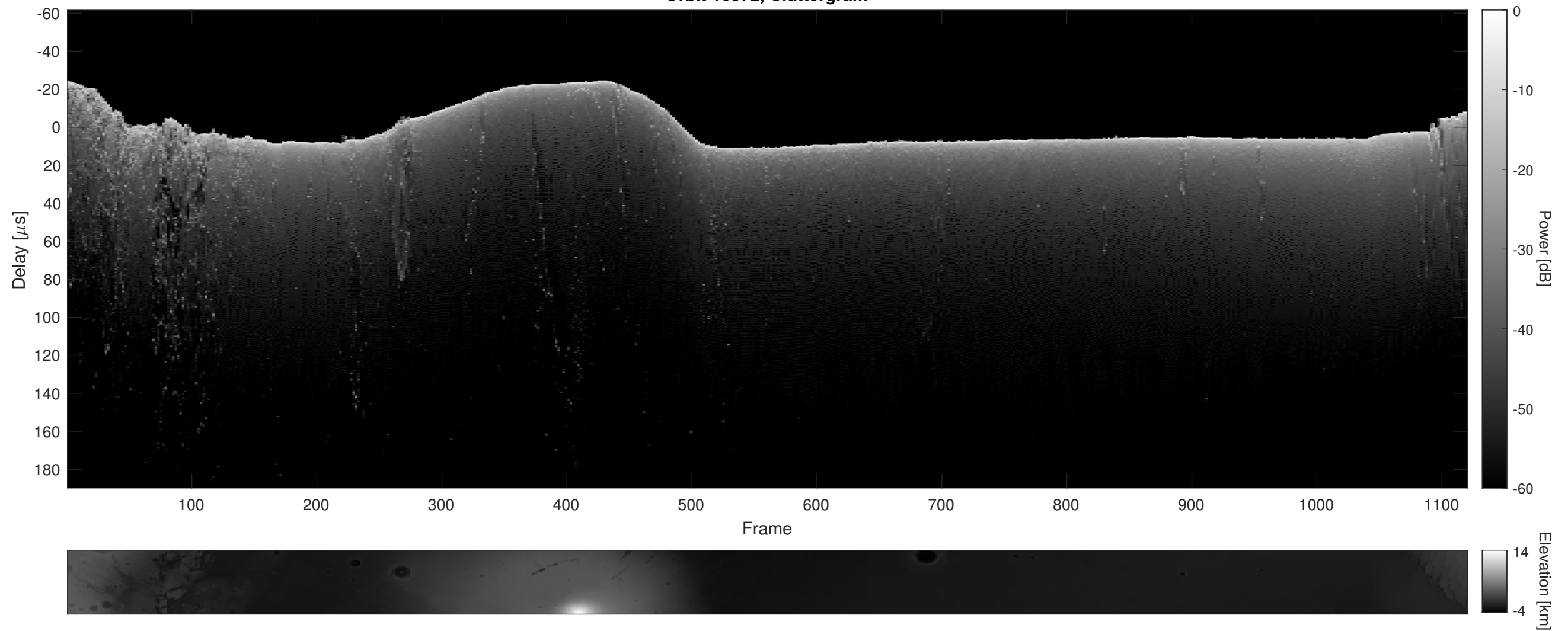
Orbit 16372, Cluttergram
