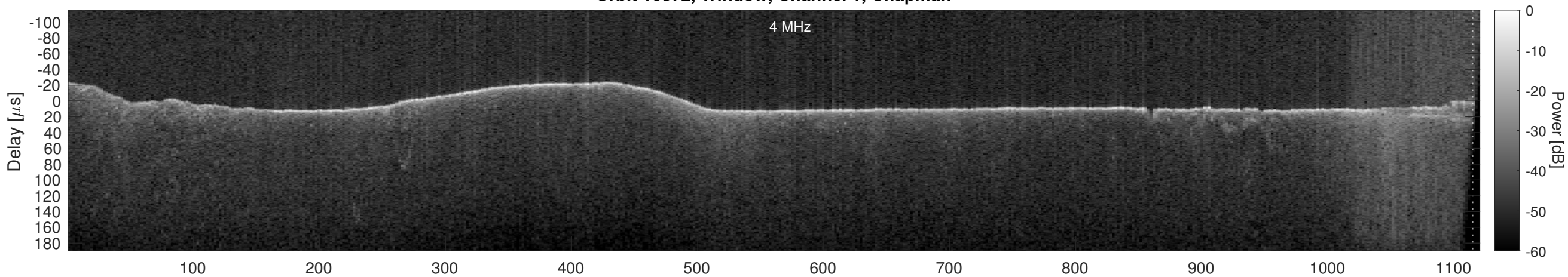
Orbit 16372, Window, Channel 1, Optimized
