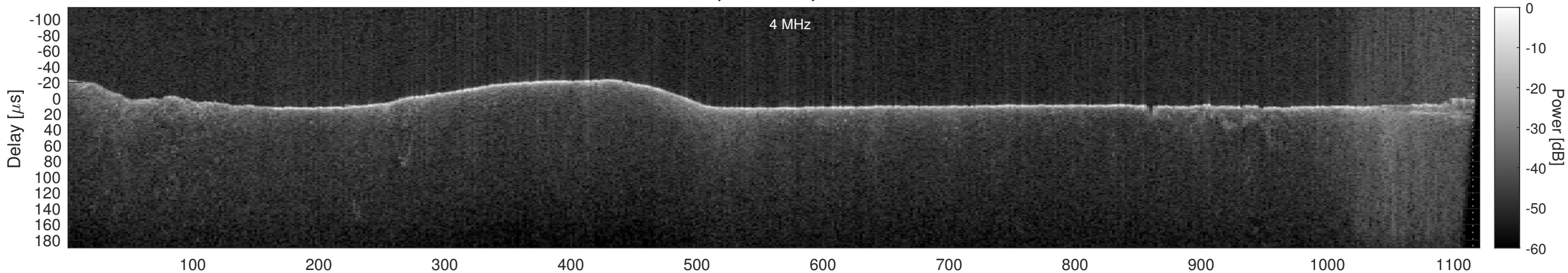
Orbit 16372, Window, Channel 1, Chapman
