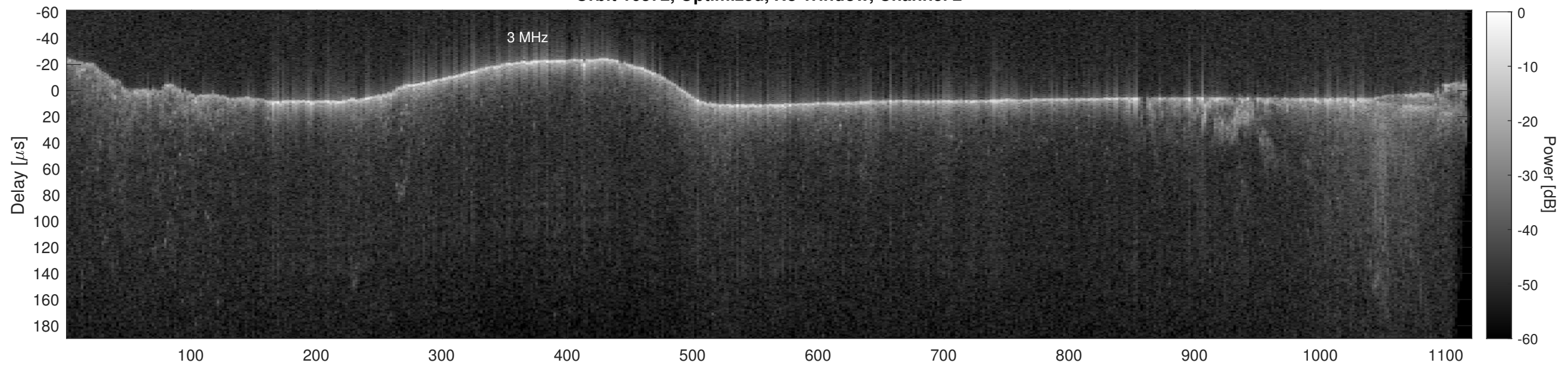
Orbit 16372, Cluttergram
