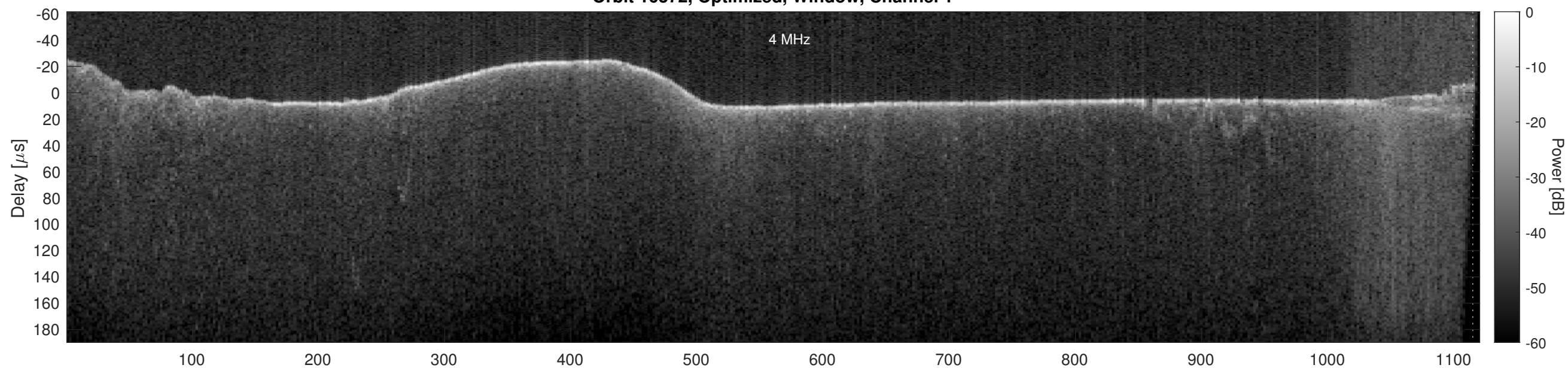
Orbit 16372, Optimized, Window, Channel 2
