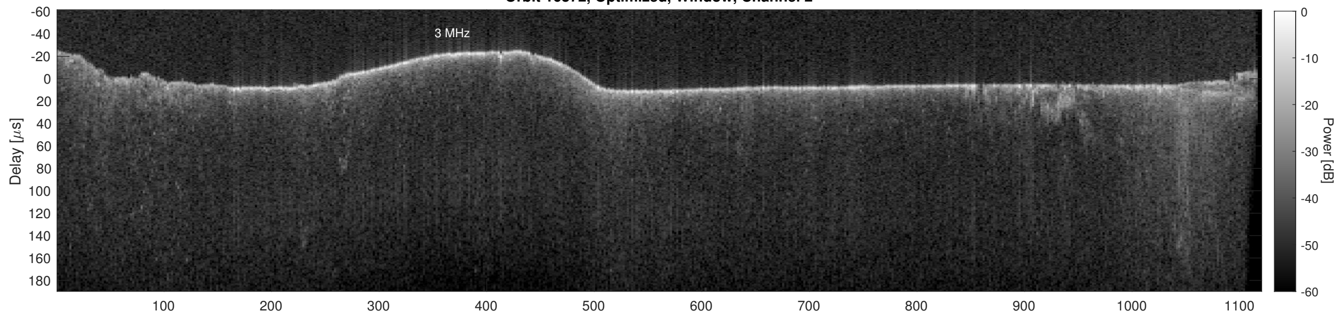
Orbit 16372, Cluttergram
