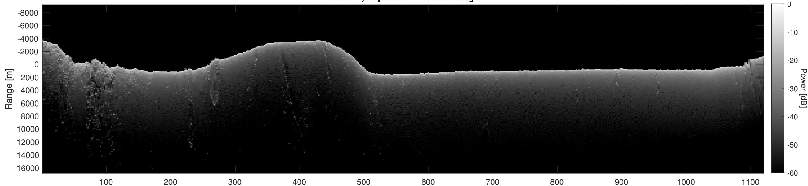
Orbit 16372, Depth-Corrected Cluttergram
