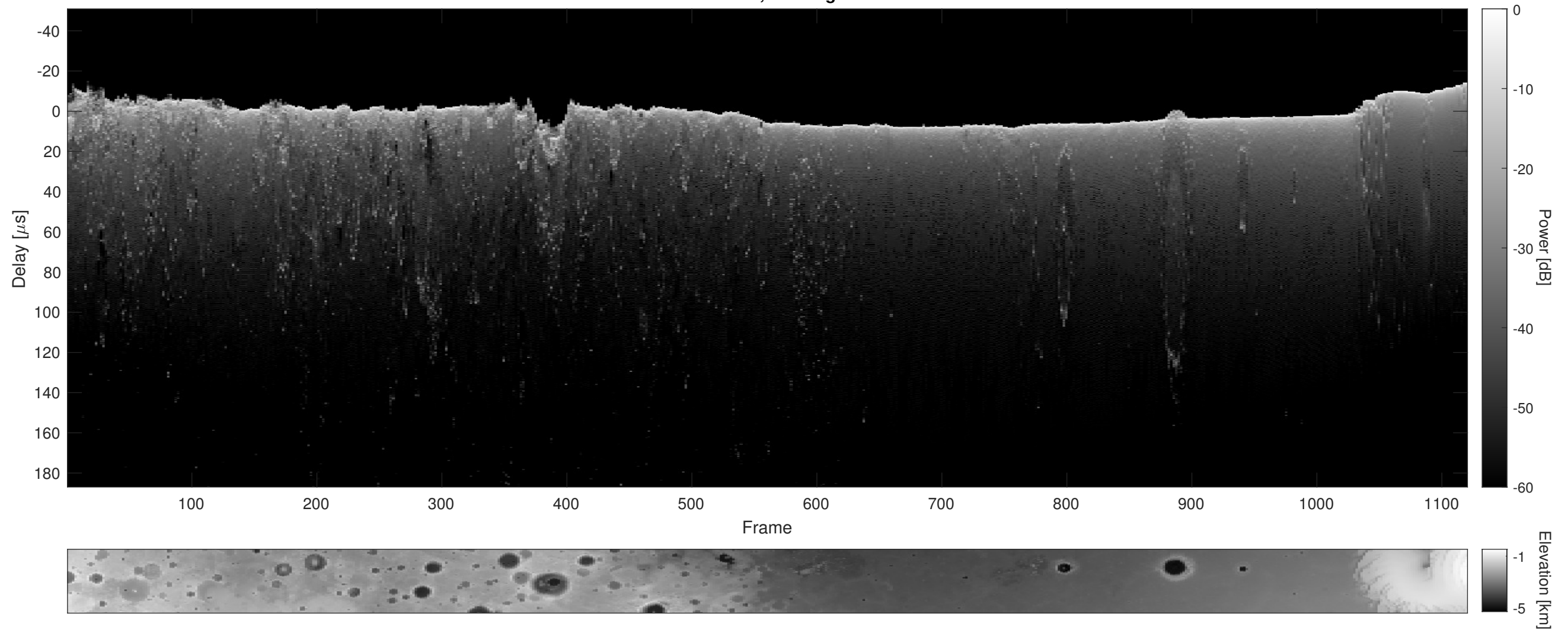
Orbit 16377, Cluttergram
