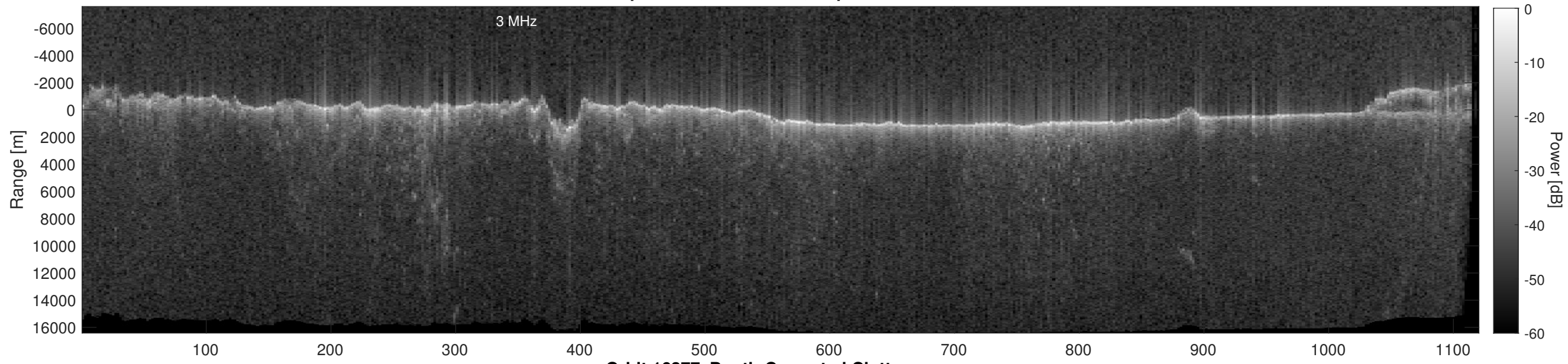
Orbit 16377, Depth-Corrected Cluttergram
