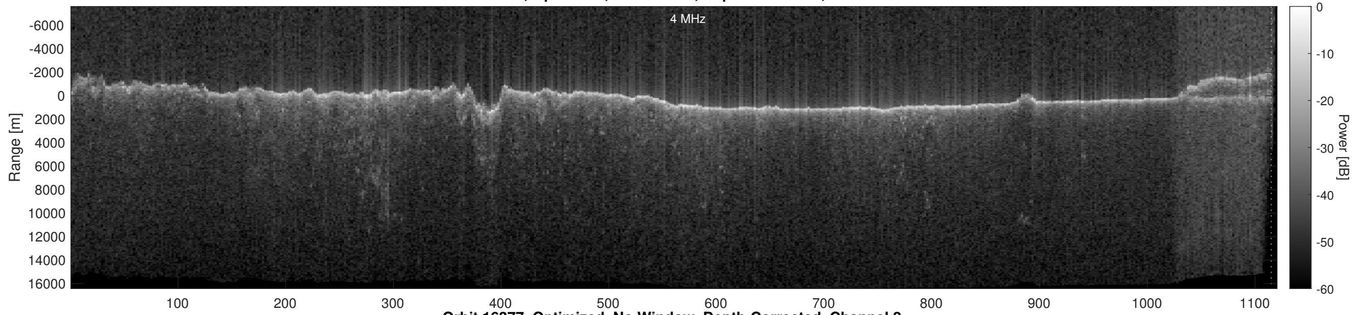
Orbit 16377, Optimized, No Window, Depth-Corrected, Channel 2
