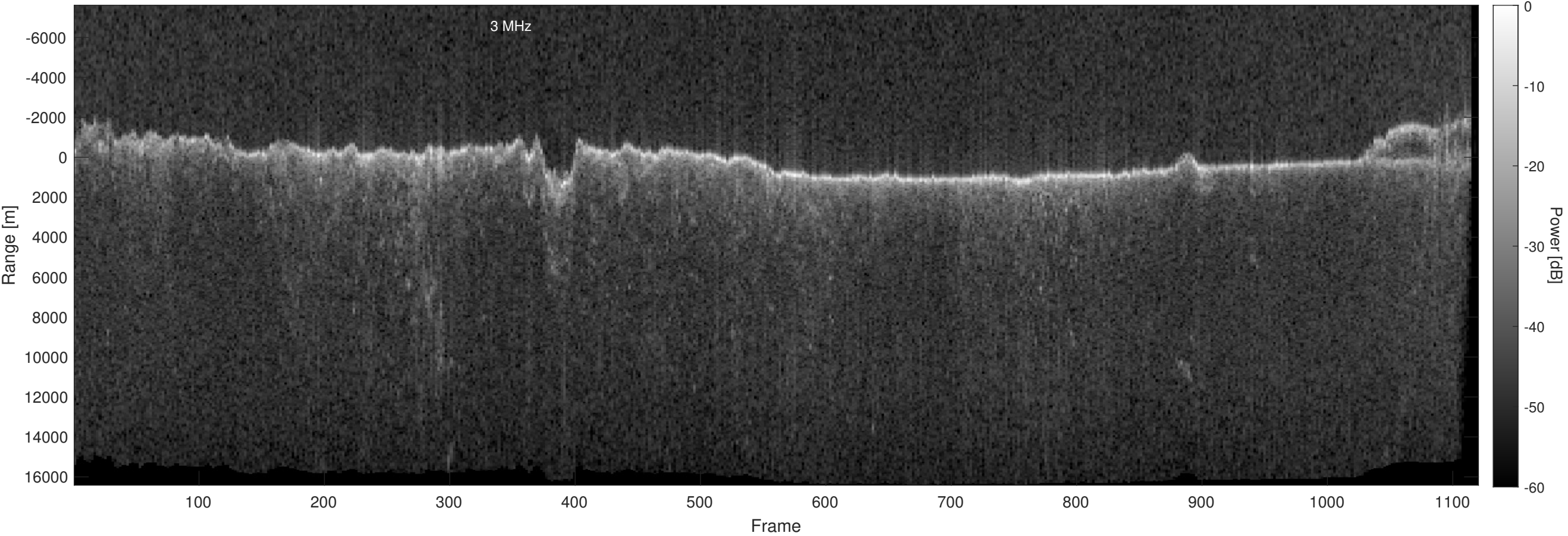
Orbit 16377, Optimized, Window, Depth-Corrected, Channel 2
