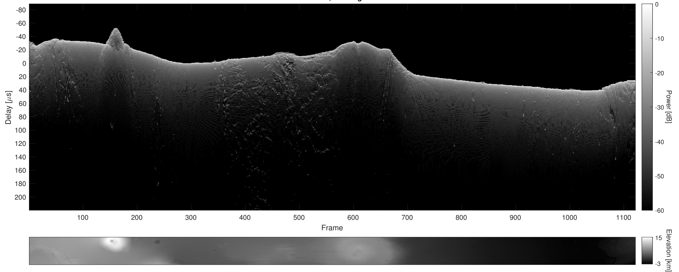
Orbit 16378, Cluttergram
