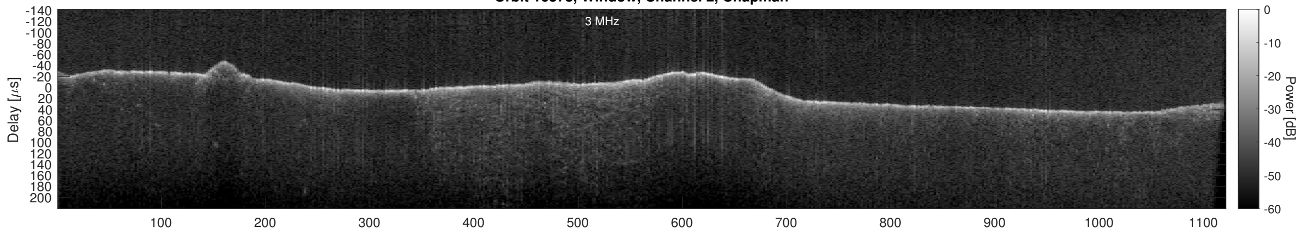
Orbit 16378, Window, Channel 2, Optimized
