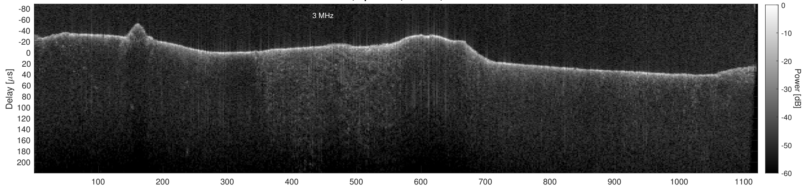
Orbit 16378, Cluttergram
