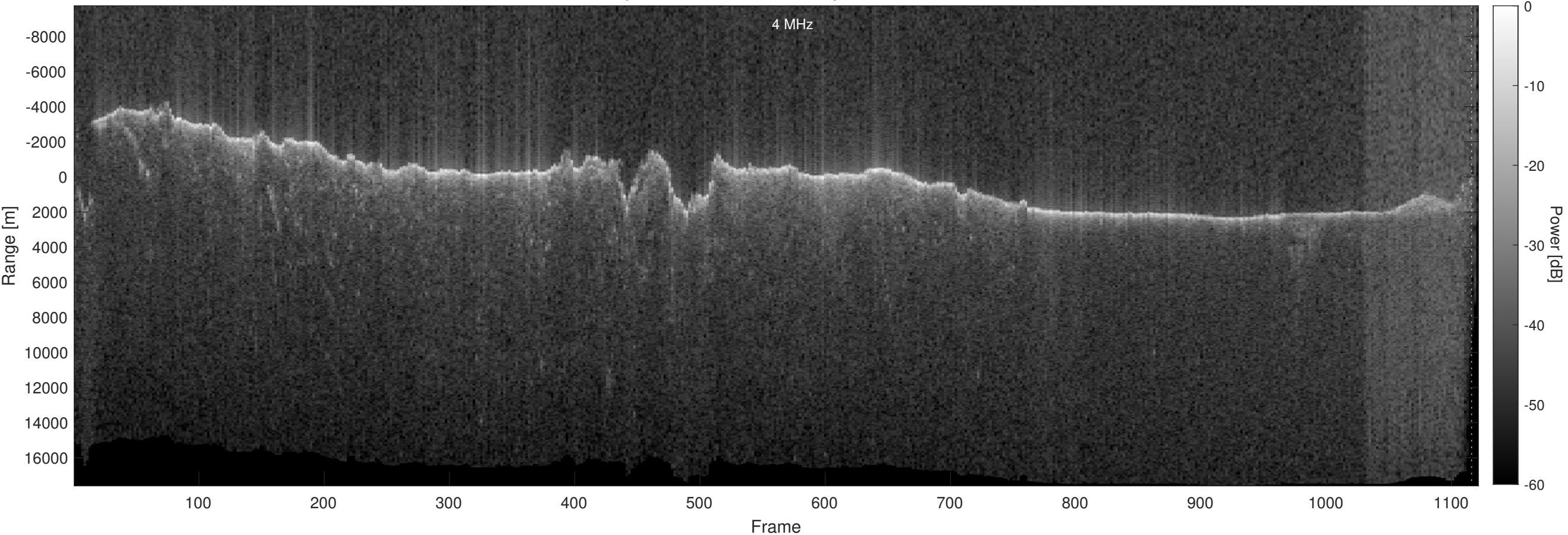
Orbit 16381, Optimized, No Window, Depth-Corrected, Channel 2
