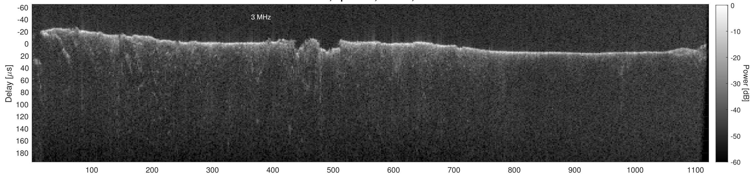
Orbit 16381, Cluttergram
