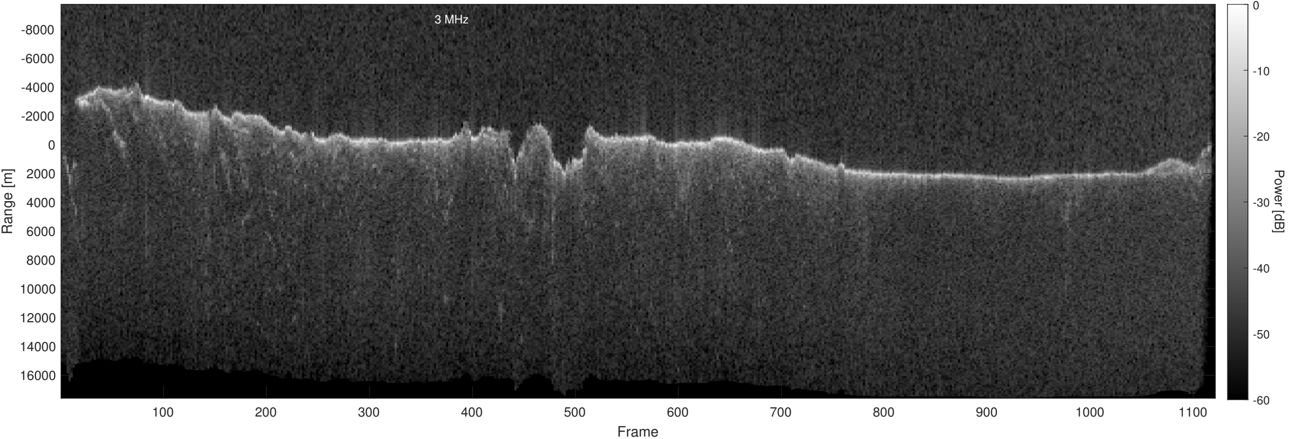
Orbit 16381, Optimized, Window, Depth-Corrected, Channel 2
