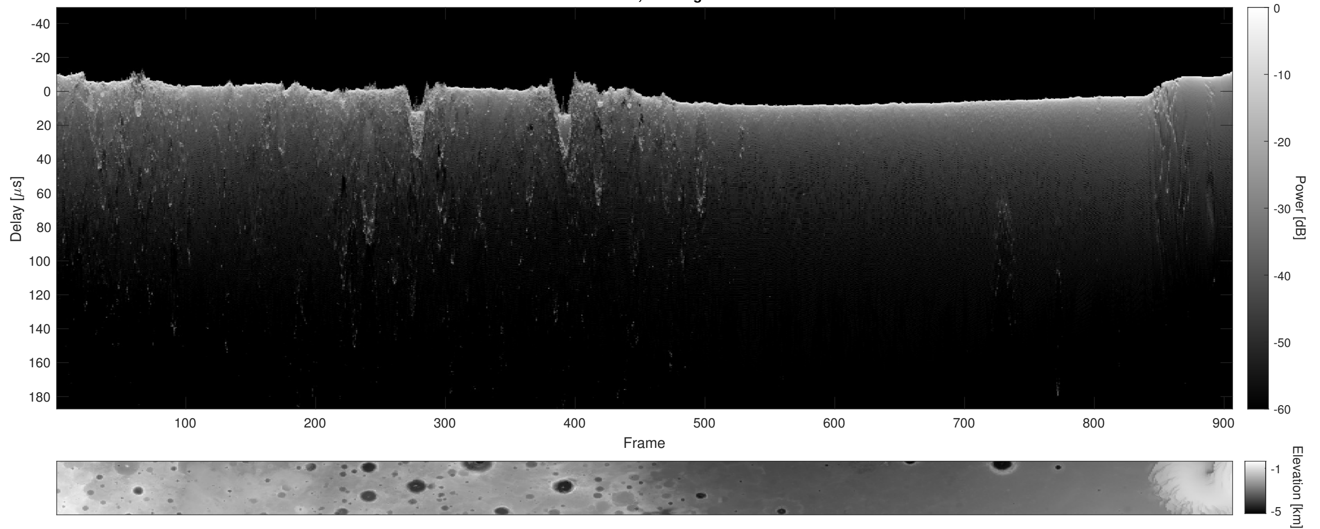
Orbit 16384, Cluttergram
