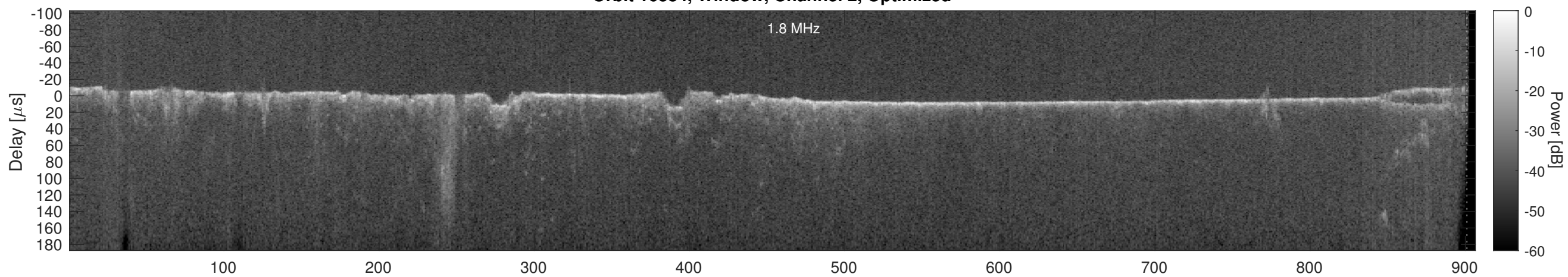
Orbit 16384, Cluttergram
