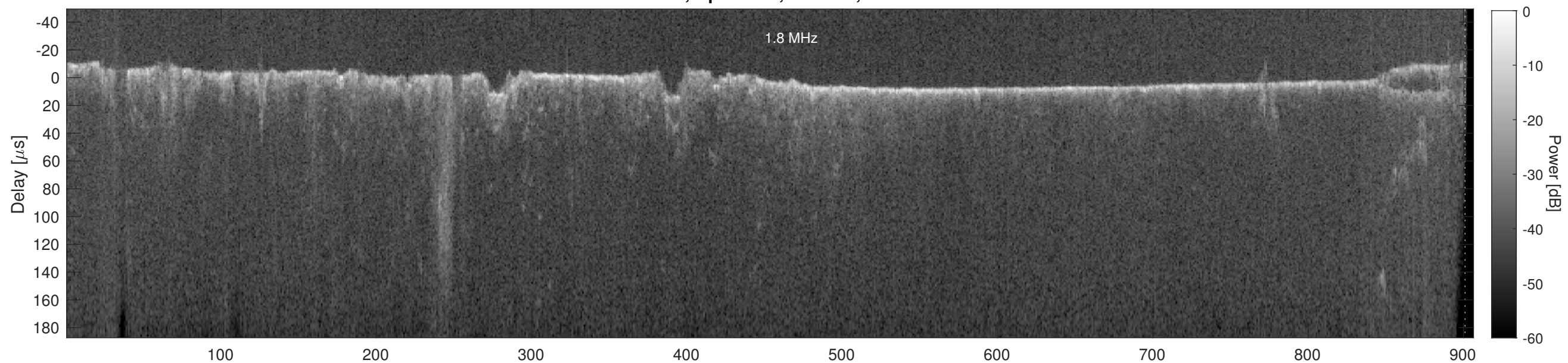
Orbit 16384, Cluttergram
