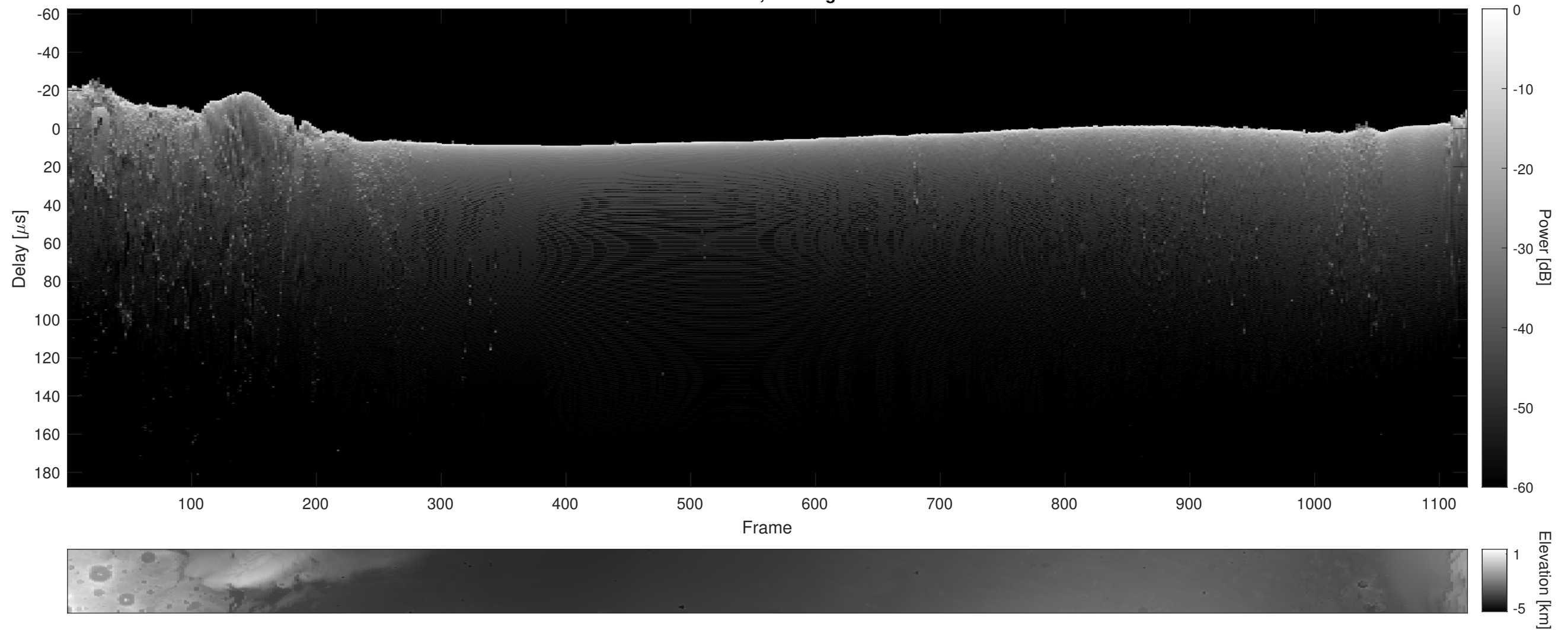
Orbit 16389, Cluttergram
