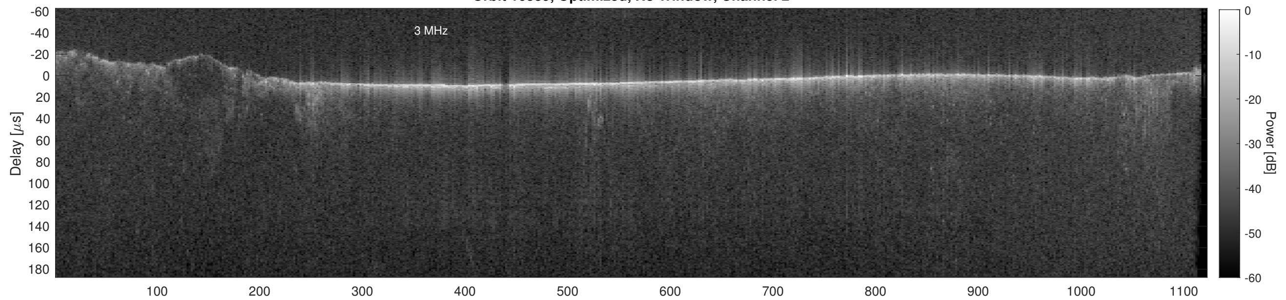
Orbit 16389, Cluttergram
