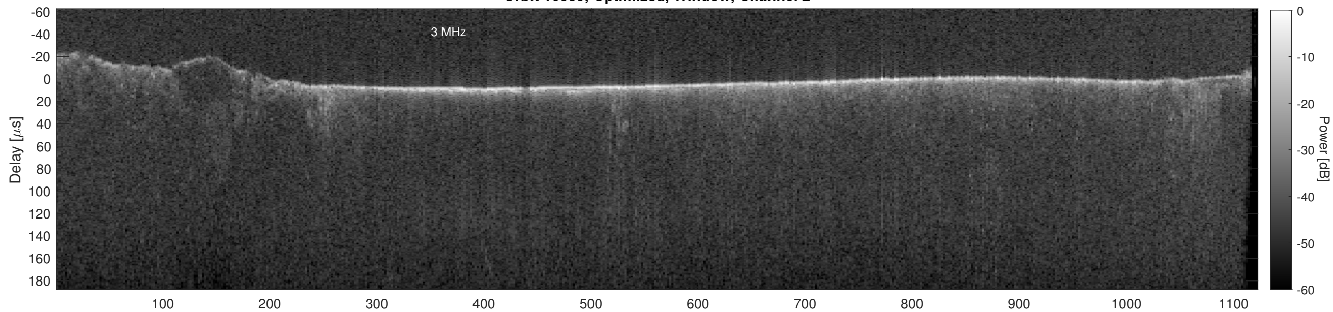
Orbit 16389, Cluttergram
