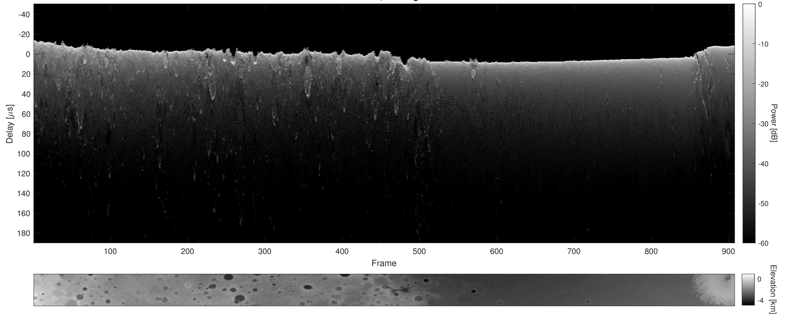
Orbit 16391, Cluttergram
