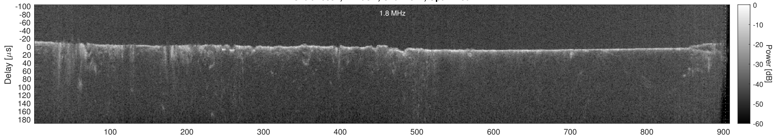
Orbit 16391, Cluttergram
