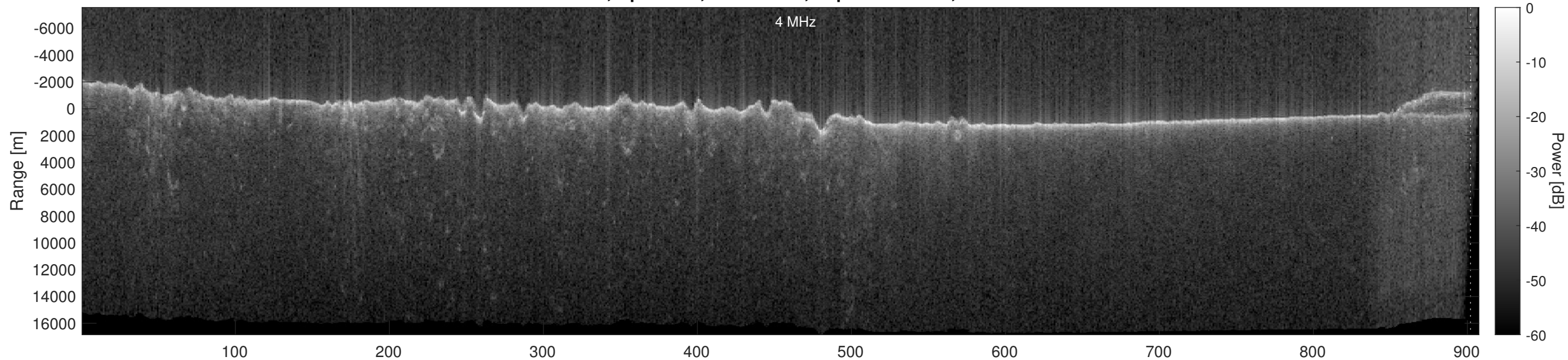
Orbit 16391, Optimized, No Window, Depth-Corrected, Channel 2
