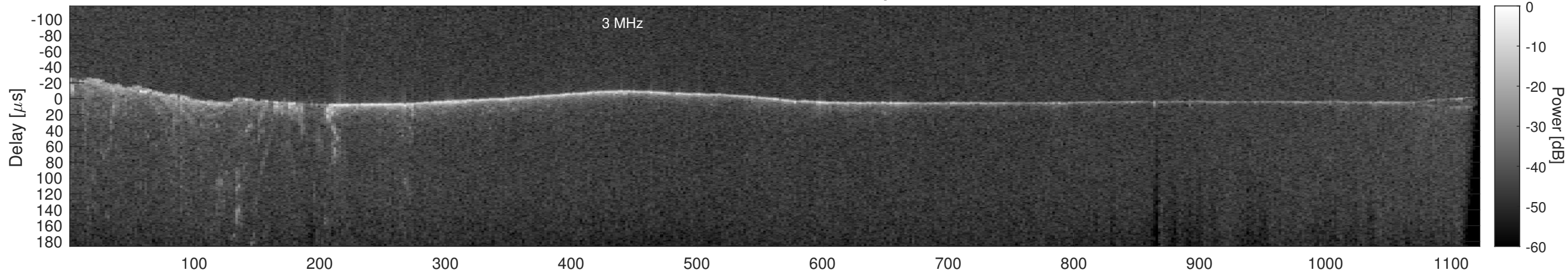
Orbit 16393, Cluttergram
