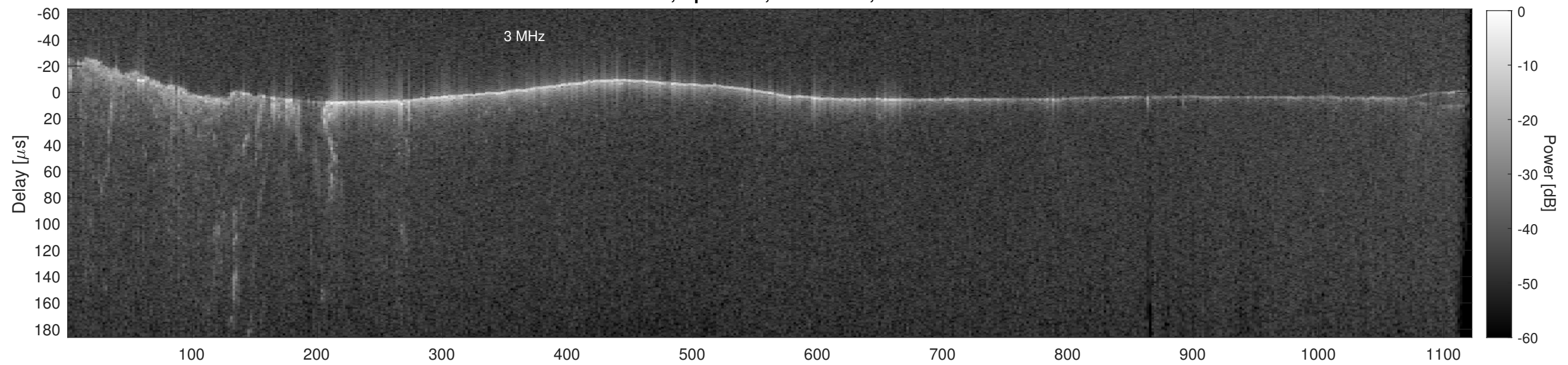
Orbit 16393, Cluttergram
