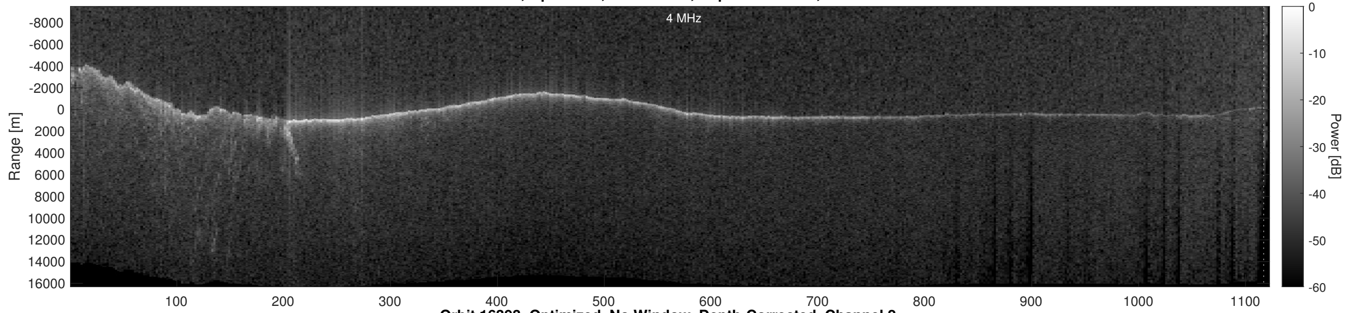
Orbit 16393, Optimized, No Window, Depth-Corrected, Channel 2
