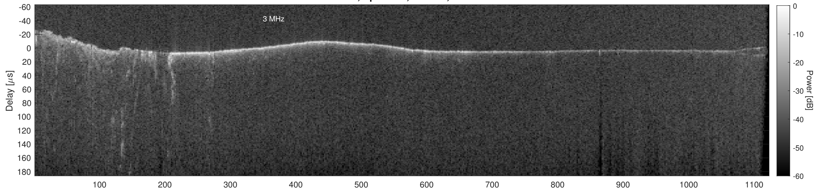
Orbit 16393, Cluttergram
