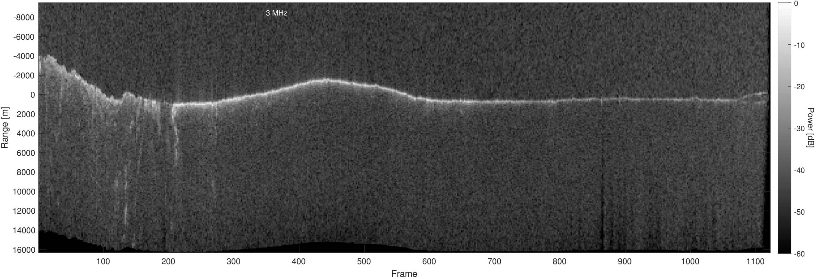
Orbit 16393, Optimized, Window, Depth-Corrected, Channel 2
