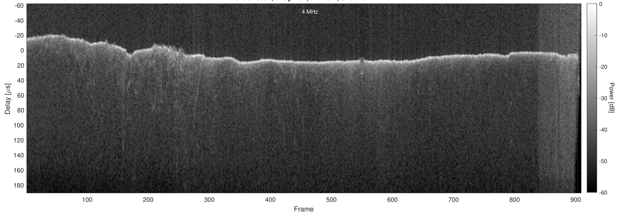
Orbit 16397, Chapman, Window, Channel 2
