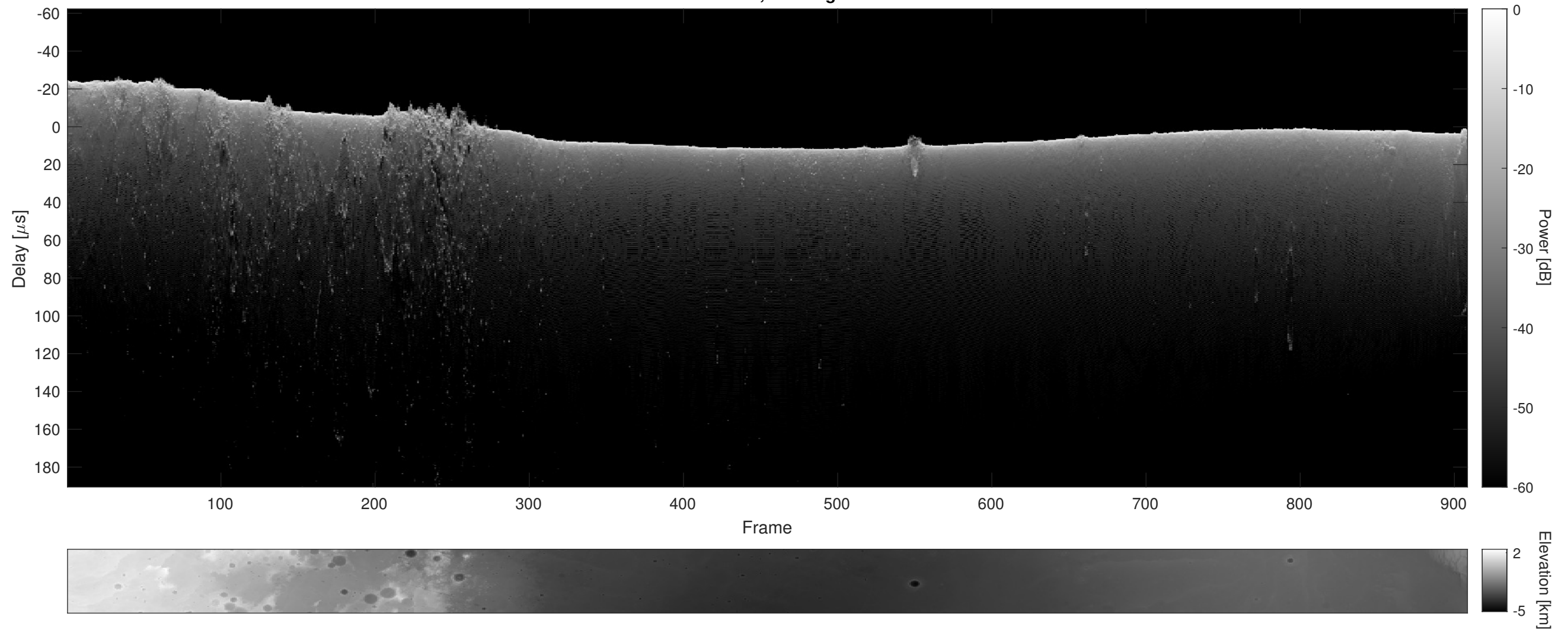
Orbit 16397, Cluttergram
