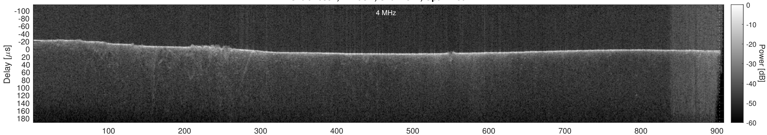
Orbit 16397, Cluttergram
