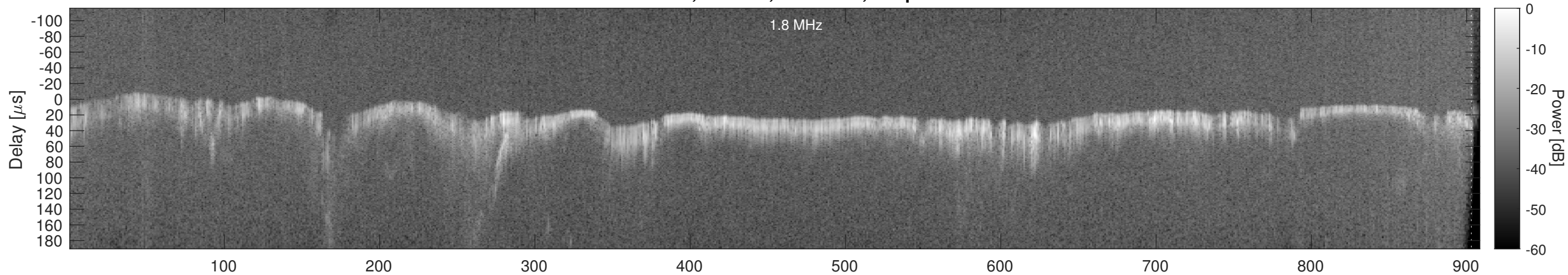
Orbit 16397, Window, Channel 2, Optimized
