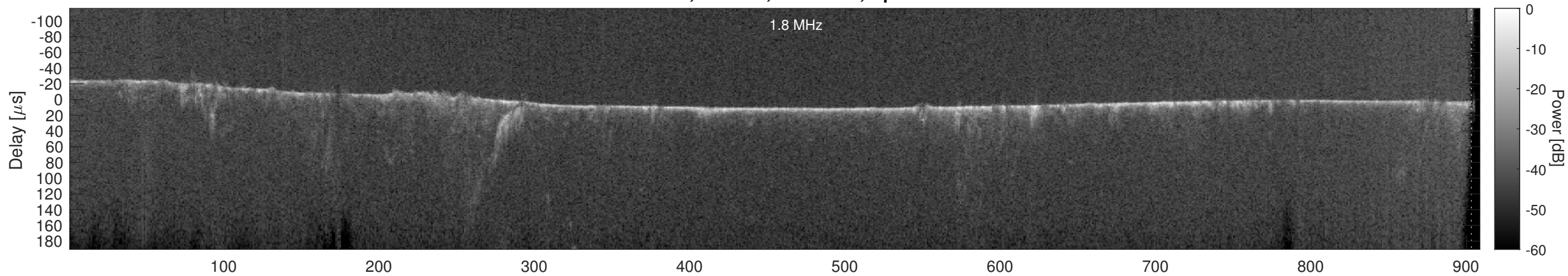
Orbit 16397, Cluttergram
