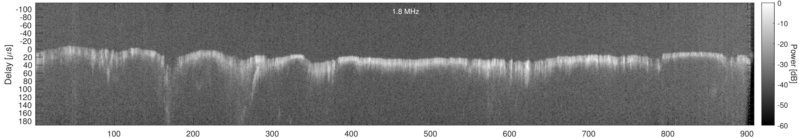
Orbit 16397, Window, Channel 2, Chapman
