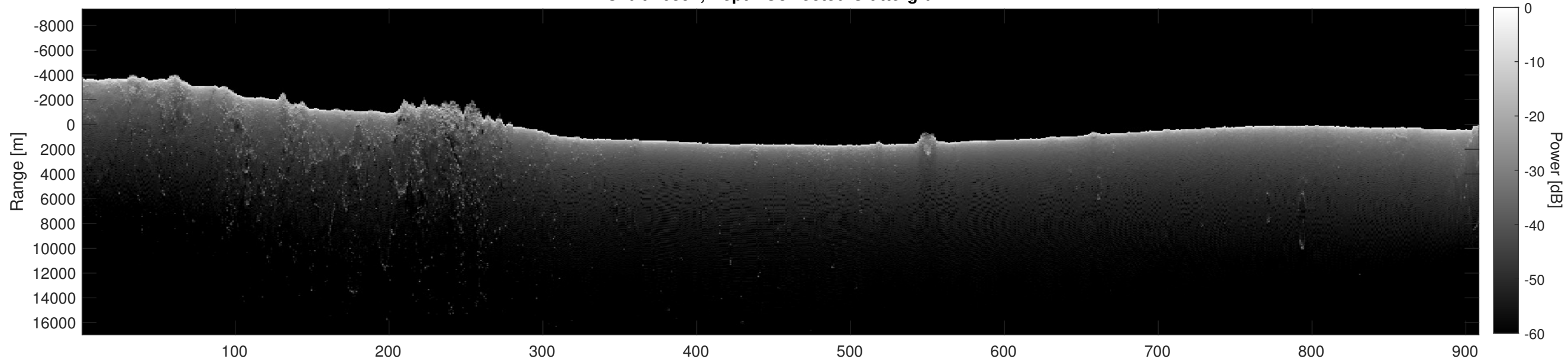
Orbit 16397, Depth-Corrected Cluttergram
