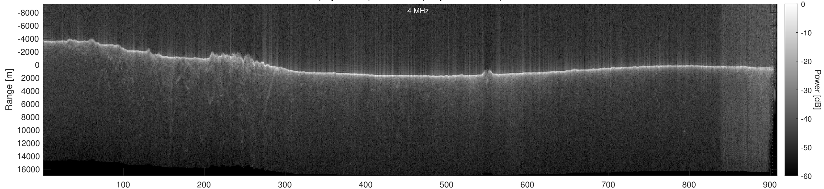
Orbit 16397, Optimized, No Window, Depth-Corrected, Channel 2
