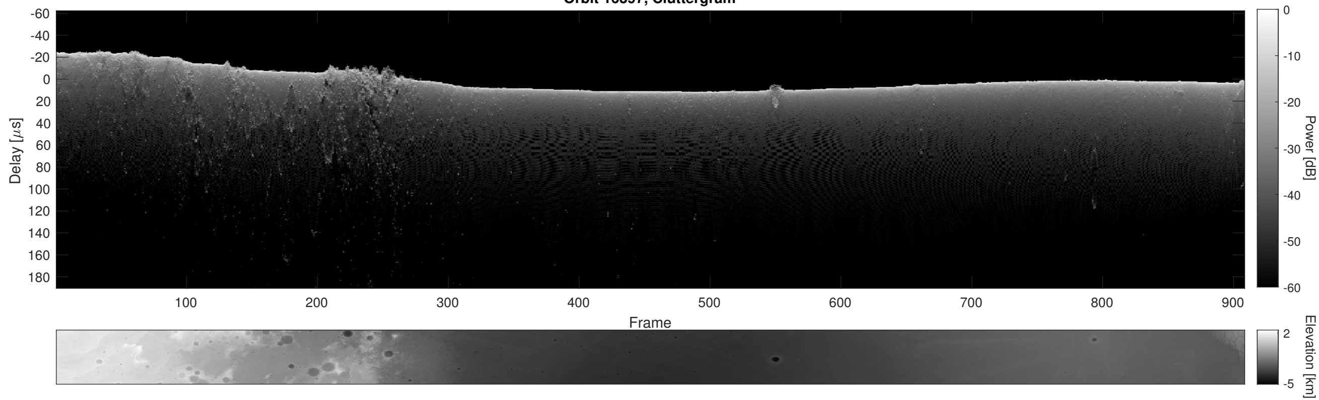
Orbit 16397, Cluttergram
