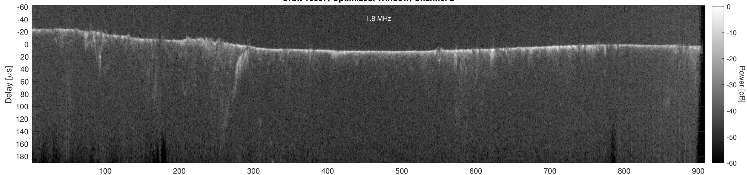
Orbit 16397, Cluttergram
