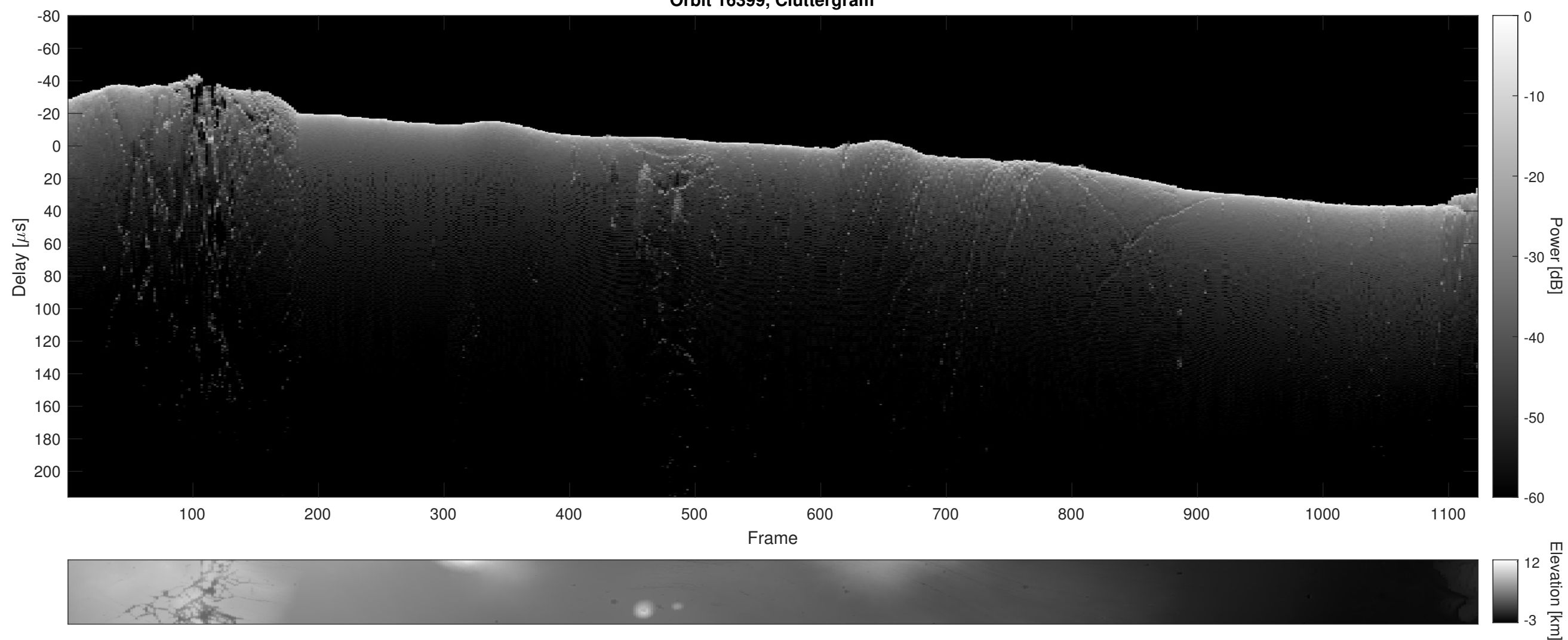
Orbit 16399, Cluttergram
