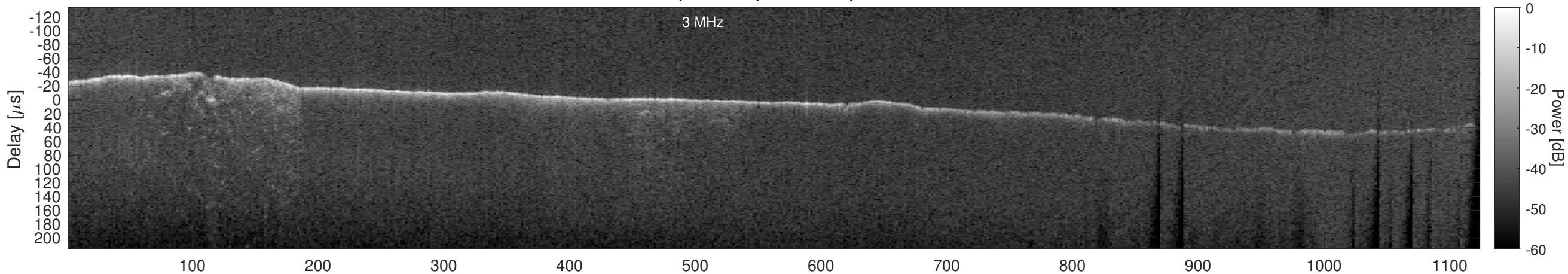
Orbit 16399, Window, Channel 2, Chapman
