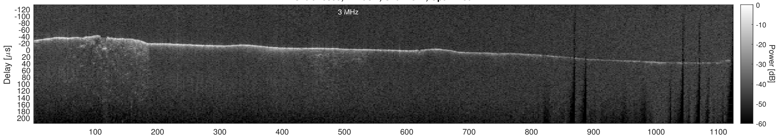
Orbit 16399, Cluttergram
