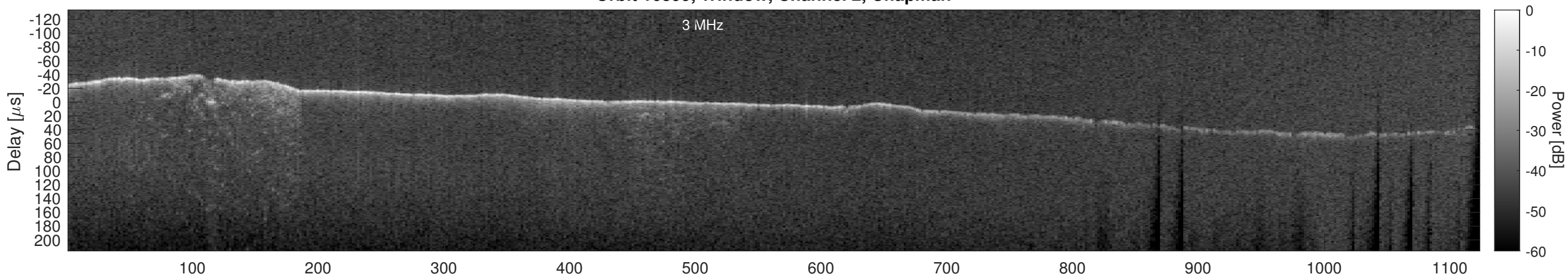
Orbit 16399, Window, Channel 2, Optimized
